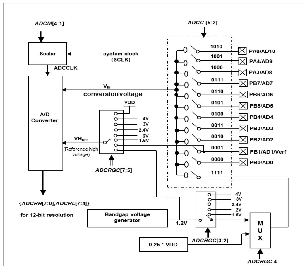
Fig. 19: ADC Block Diagram
