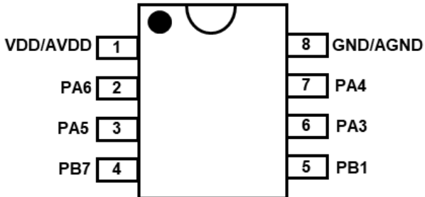
PFS122B-S08 (SOP8-150mil)
