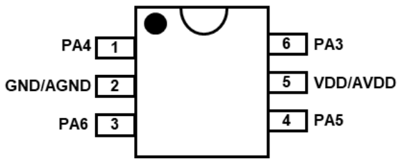
PFS122B-U06 (SOT23-6 60mil)
