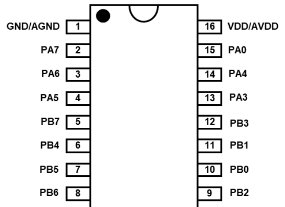
PFS122B-S16B (SOP16B-150mil)
