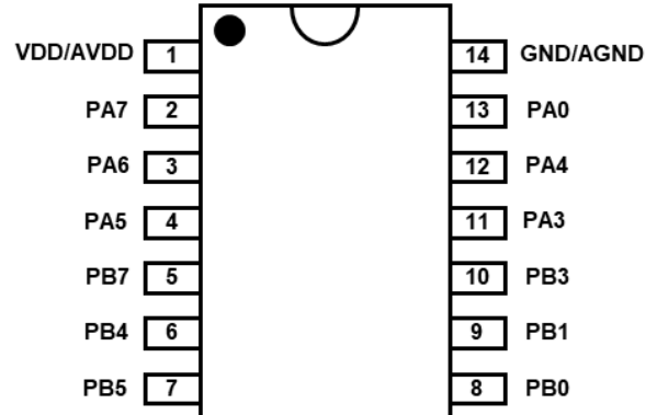
PFS122B-S14 (SOP14-150mil)
