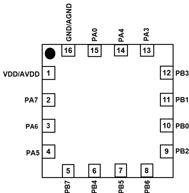
PFS122B-1J16A (QFN3*3-16pin-0.5pitch)
