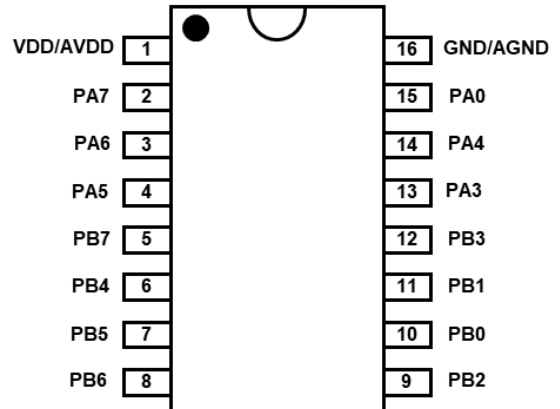
PFS122B-S16A (SOP16A-150mil)
